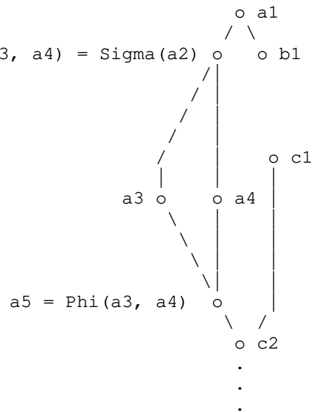
Data-flow graph in SSI form
